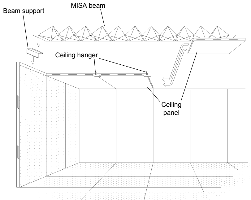
Ceiling hanger kit installation (shown with MISA beam)
