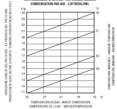
RAFFREDDAMENTO AD ARIA - AIR COOLED MODELS CONDENSATION PAR AIR - LUFTKÜHLUNG
