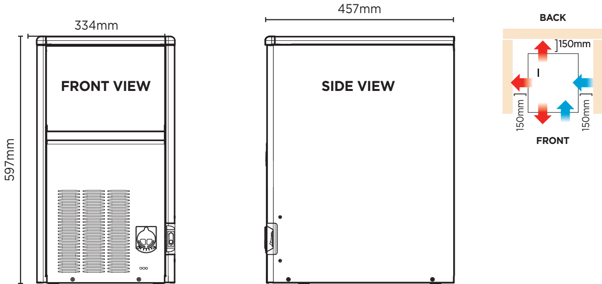
RAFFREDDAMENTO AD ARIA - AIR COOLED MODELS CONDENSATION PAR AIR - LUFTKÜHLUNG
